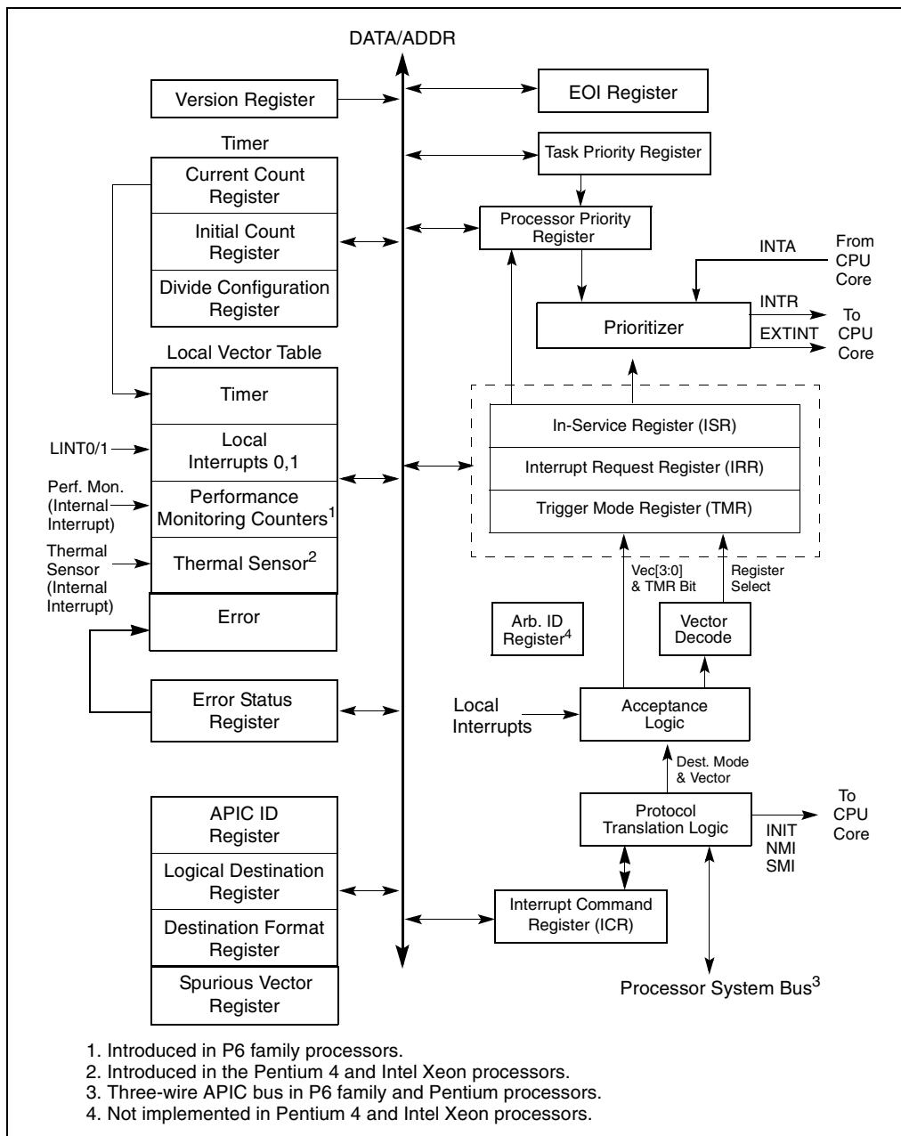
Figure 8-4. Local APIC Structure
