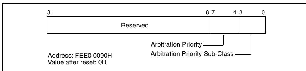
Figure 8-15. Arbitration Priority Register (APR)
