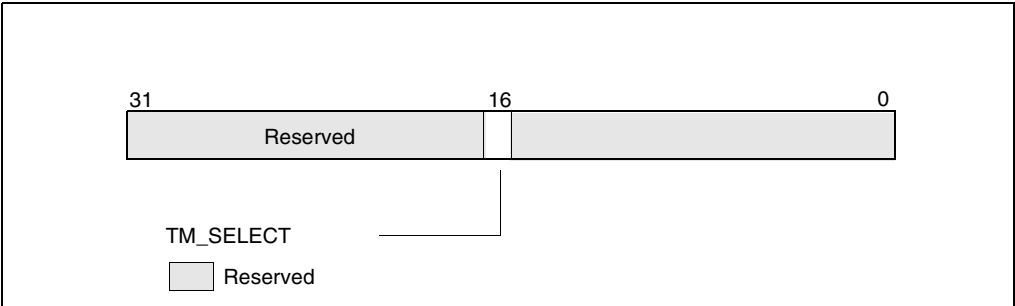
Figure 13-7. MSR_THERM2_CTL Register for the Pentium M Processor
