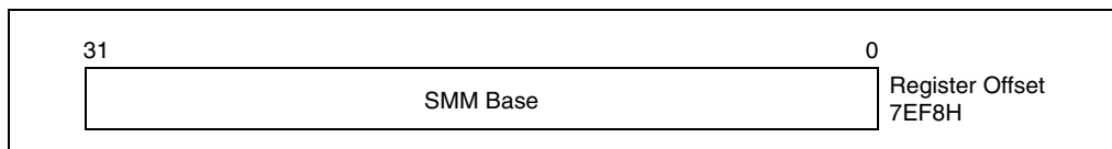
Figure 13-4. SMBASE Relocation Field
