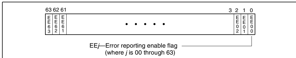
Figure 14-5. IA32_MCi_CTL Register
