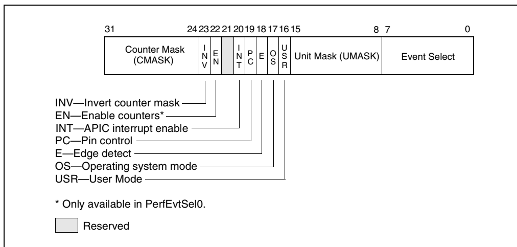
Figure 15-19. PerfEvtSel0 and PerfEvtSel1 MSRs
