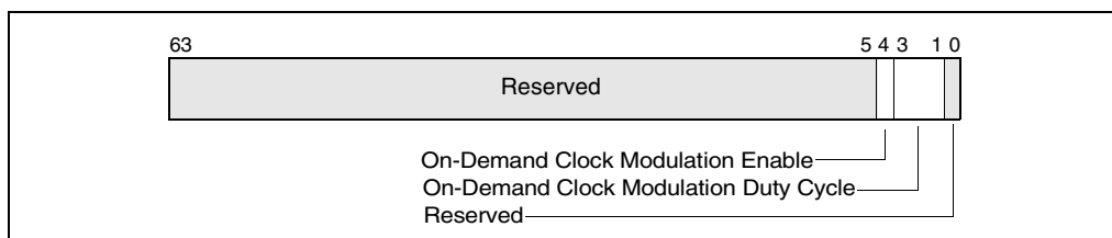
Figure 13-11. IA32_CLOCK_MODULATION MSR
