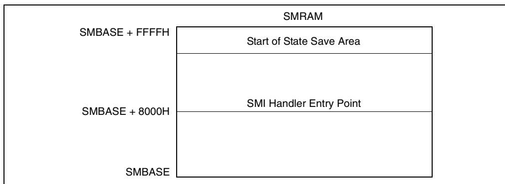
Figure 13-1. SMRAM Usage
