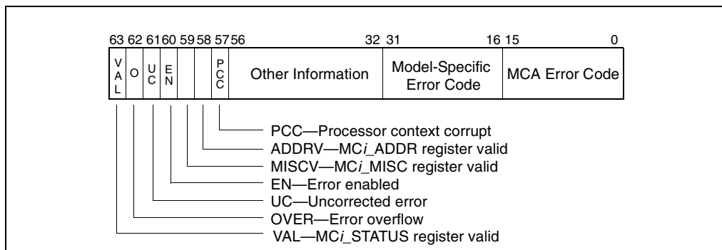
Figure 14-6. IA32_MCI_STATUS Register
