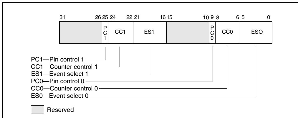
Figure 15-20. CESR MSR (Pentium Processor Only)
