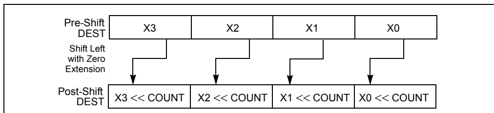
Figure 4-7. PSLLW, PSLLD, and PSLLQ Instruction Operation Using 64-bit Operand
