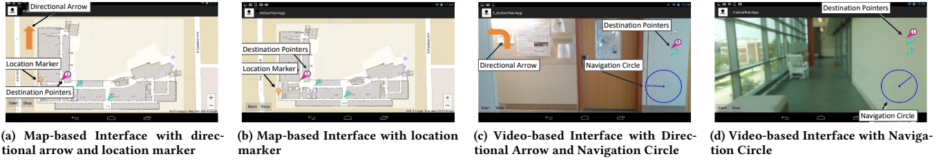
Figure 3: Map-based interfaces with (a) a directional arrow and a location marker (b) a location marker. Video-based interface with (c) a directional arrow and a navigation circle, (d) a navigation circle. We used the directional arrow to provide turn-by-turn directions to assist users in their navigation tasks. The location marker and the navigation circle were updated after every step to provide relative location updates suitable for the background reference frame. The map shown in map-based interfaces was the simple version of the original floor plan where we grayed out all the rooms since participants did not have access to any rooms. They could only access the hallways during the user study.
