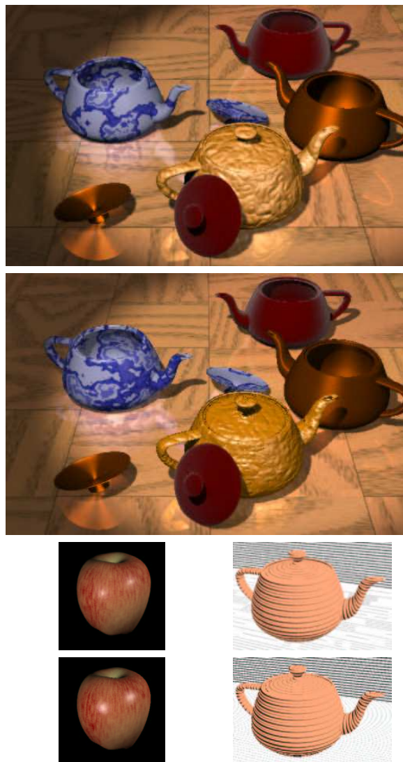
Figure 4: RenderMan SL Examples. The top and bottom images of each pair were rendered with PhotoRealistic RenderMan from Pixar and our multi-pass OpenGL renderer, respectively. No shaders use image maps, except for the reflection and depth shadow maps generated on the fly. The wood floor, blue marble, red apple, and wood block print textures all are generated procedurally. The velvet and brushed metal shaders use sophisticated illuminance blocks for their reflective properties. The specular highlight differences are due to Pixar's proprietary specular function; we use the definition from the RenderMan specification. The blue marble, wood floor, and apple do not match because of differences in the noise function. Other discrepancies typically are due to limited precision lookup tables used to help evaluate mathematical functions. (Credit: LGParquetPlank by Larry Gritz, SHWvelvet and SHWbrushedmetal by Stephen Westin, DPBlueMarble by Darwin Peachey, eroded from the RenderMan companion, JMredapple by Jonathan Merritt, and woodblockprint by Scott Johnston. Courtesy of the RenderMan Repository http://www.renderman.org .)
