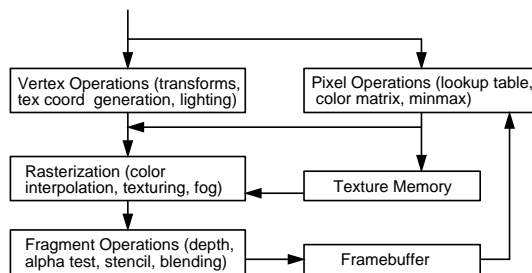
Figure 1: A simplified block diagram of the OpenGL architecture. Geometric data passes through the vertex operations, rasterization, and fragment operations to the framebuffer. Pixel data (either from the host or the framebuffer) passes through the pixel operations and on to either texture memory or through the fragment pipeline to the framebuffer.
