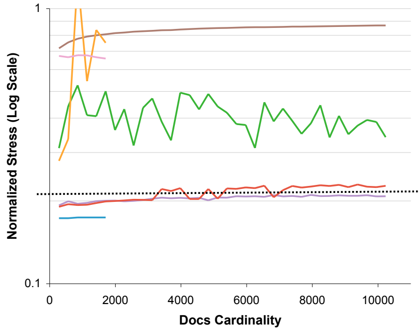
Glimmer (8800GTX) GPU-SF (8800GTX) Glimmer (7900GS) GPU-SF (7900GS) PivotMDS Hybrid CPU-SF Classic SMACOF
