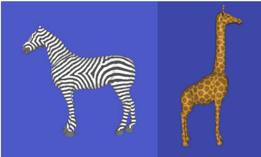
Turk, SIGGRAPH 91
