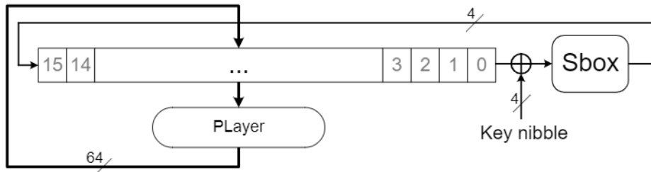
Figure 4: Nibble-serial architecture of the PRESENT block cipher, key schedule not shown.
