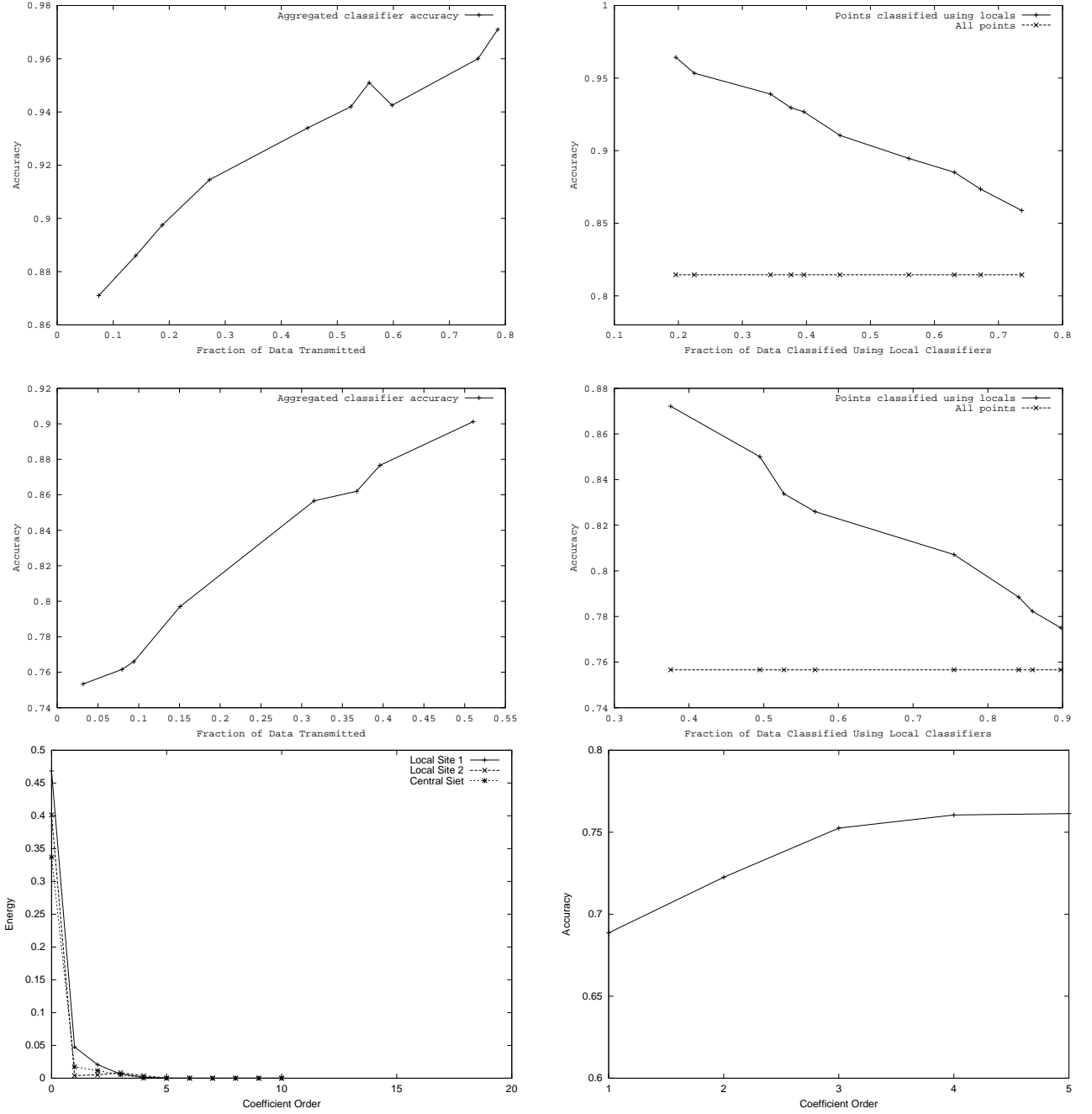
Figure 8: The Figures (left to right and top to bottom) are: a. Accuracy vs. transmission for Quest data, b. Accuracy of local models vs. 0 classified by them, c. Accuracy vs. transmission for Gene data, d. Accuracy of local models vs. instances classified by them, e. Energy of coefficients vs. their order, f. Accuracy of Fourier Representation based model vs. order of coefficients used.
