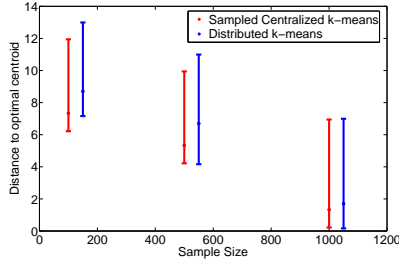
(a) Average Quality vs. Sample Size
