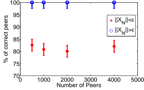
(a) Average quality vs. number of peers
