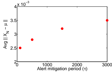
(a) Quality vs. \tau
