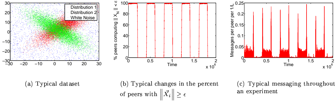
Figure 2: A typical experiment is run for 10 equal length epochs. The epochs have very similar means, and very large variance. Quality and overall cost are measured across the entire experiment. The monitoring cost is measured on the last 80% of every epoch, in order to ignore transitional effects.
