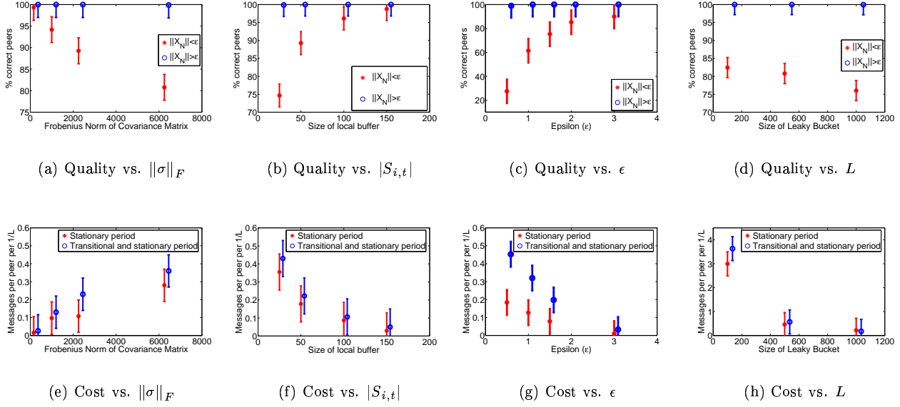
Figure 3: Dependency of cost and quality of L2 Thresholding on \|\sigma\|_F , |S_{i,t}| , \epsilon , and L . Quality is defined by the percentage of peers correctly computing an alert (separated for epochs with \|\vec{X}_N\| less and more than \epsilon ). Cost is defined as the portion of the leaky buckets intervals that are used. Both overall cost and cost of just the stationary periods are reported.
