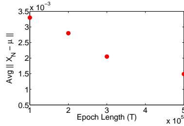
(b) Quality vs. Epoch Length
