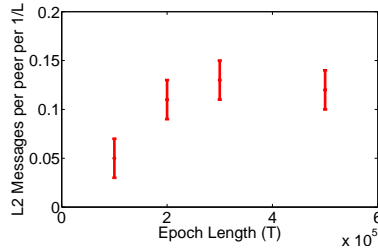
(e) Cost vs. Epoch Length
