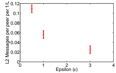
(f) Cost vs. \epsilon
