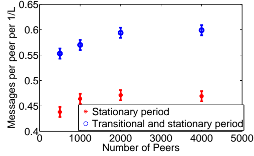
(b) Average cost vs. number of peers
